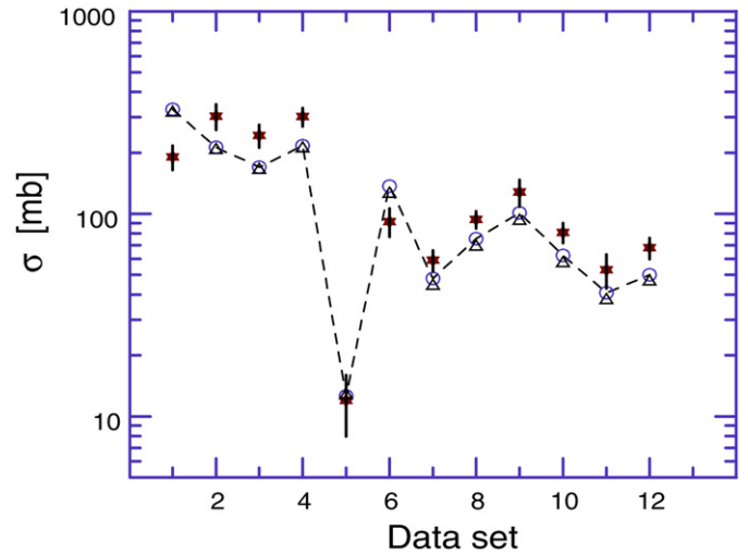
Fig. 1. Comparison between experimental Coulomb excitation cross sections (solid stars with error bars) and theoretical ones, calculated either with Eq. (3) (open circles), or with Eq. (5) (open triangles).
