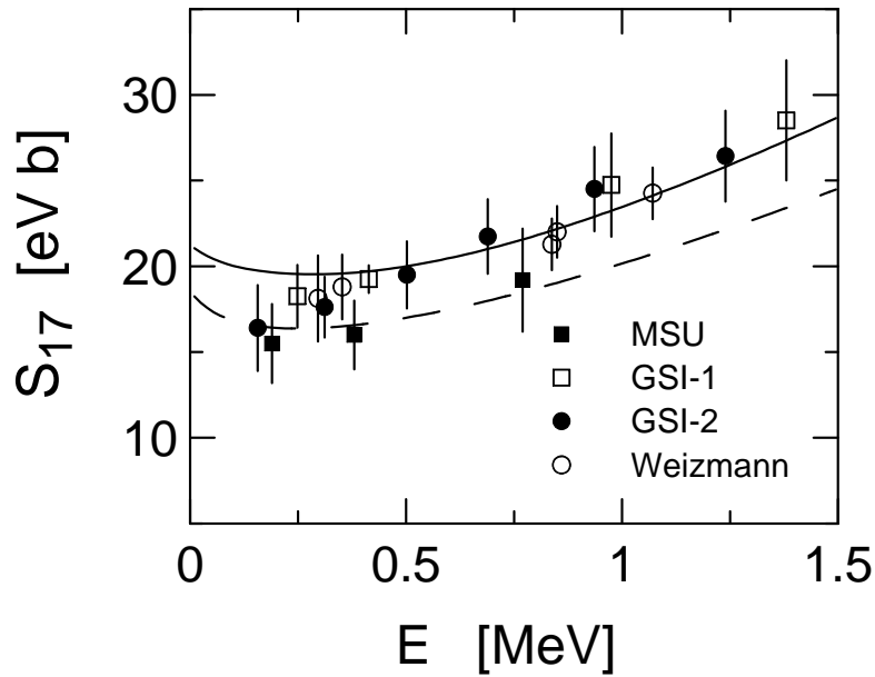
FIG. 4: Astrophysical S-factor for the reaction p+{}^8\text{B} . The data are the experimental points of recent experiments [25–28]. The solid and dashed curves are results of calculations with different choices of the Woods-Saxon potential which reproduces the binding of {}^8\text{B} .
